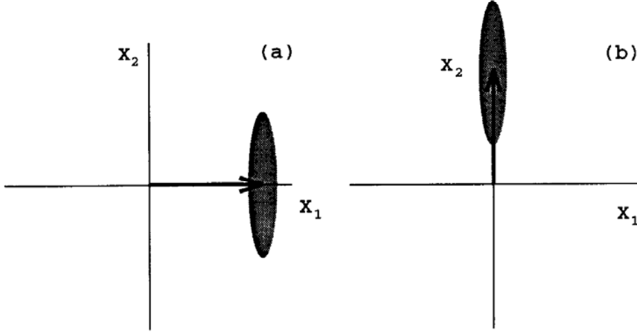
Fig. 3.4. Phase-space of amplitude and phase squeezed states. (a) The quadrature carrying the coherent excitation is squeezed ( \theta = 0 ). (b) The quadrature out of phase with the coherent excitation is squeezed ( \theta = \pi/2 )
