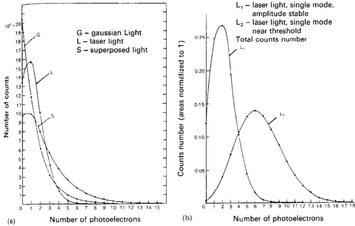
Fig. 3.2. Measured photo-count statistics for (a) Gaussian, laser and superposed fields. Measuring time of a single sample: 10 \mu\text{s} . Coherence time of the Gaussian field; 40 \mu\text{s} . (b) Two laser fields. Measuring time of a single sample: 10 \mu\text{s}
