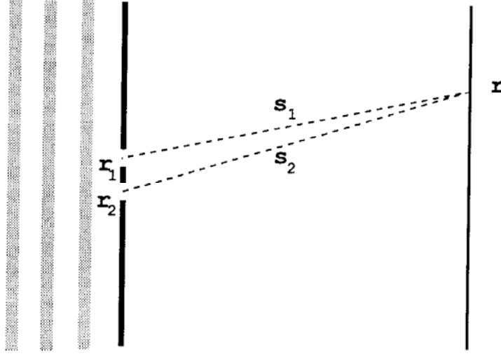
Fig. 3.1. Schematic representation of Young's interference experiment
