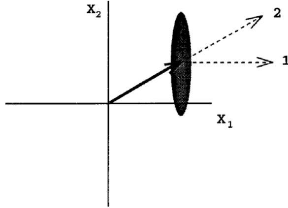
Fig. 3.3. A phase convention for squeezed states. Direction 1 is the direction of squeezing, direction 2 is the direction of coherent excitation. The error ellipse is aligned so that the squeezing direction is parallel to the X_1 direction.
